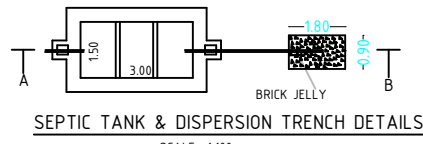
SEPTIC TANK & DISPERSION TRENCH DETAILS SCALE= 1:100
