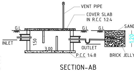
SECTION-AB
