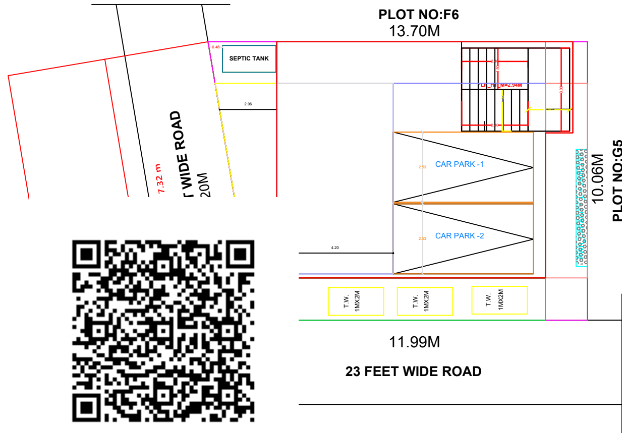
SITE CUM STILT FLOOR PLAN
