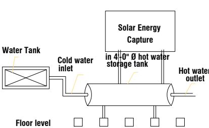
SOLAR HOT WATER SYSTEM
