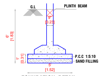
FOUNDATION DETAIL
