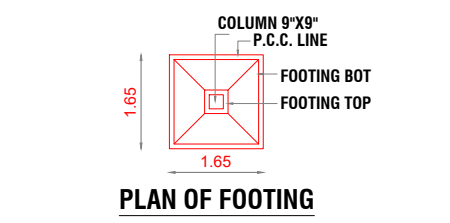
PLAN OF FOOTING
