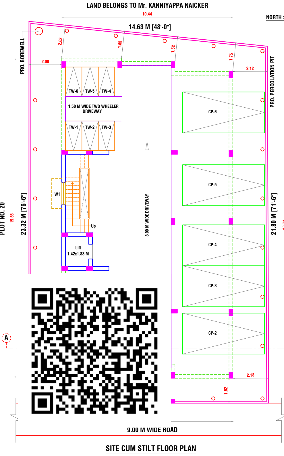
SITE CUM STILT FLOOR PLAN
