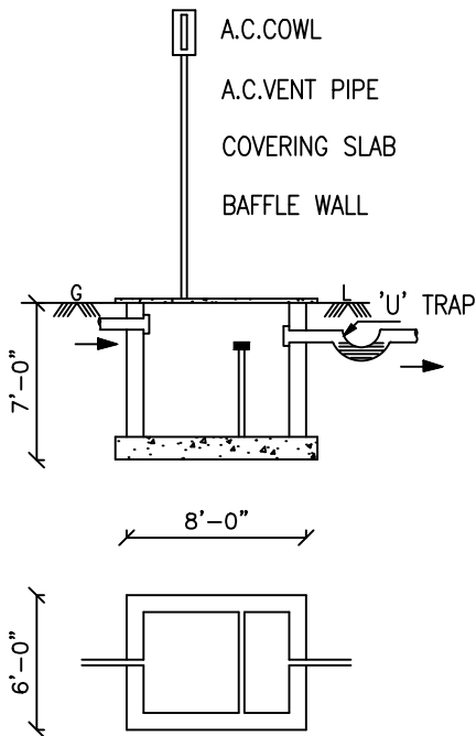
SEPTIC TANK
