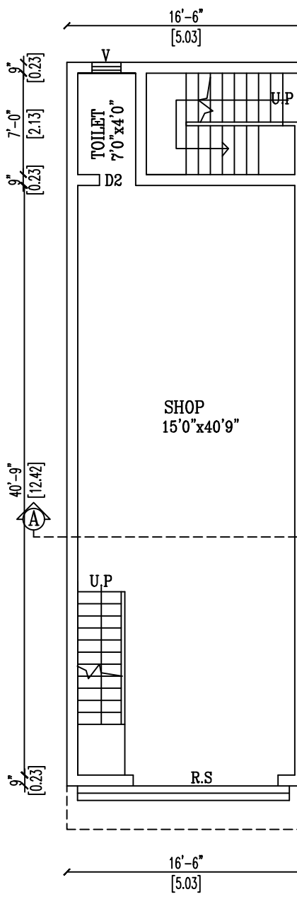
EXTG. GROUND FLOOR PLAN
