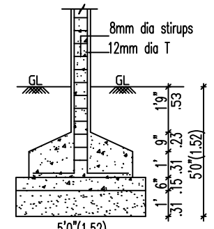
COLUMN FOUNDATION DETAIL SCALE 1"=4'0"(1:50)
