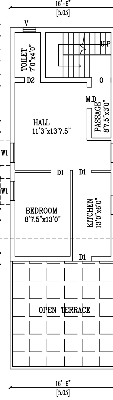
PRO. SECOND FLOOR PLAN
