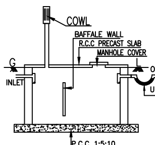
SECTION DETAILS OF SEPTIC TANK
