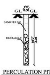
PERCOLATION PIT
