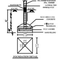
FOUNDATION DETAIL
