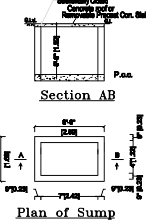
Plan of Sump
