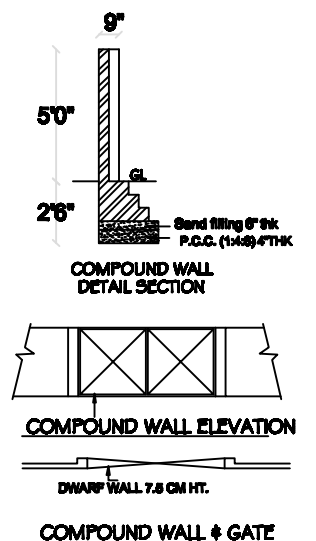
COMPOUND WALL & GATE
