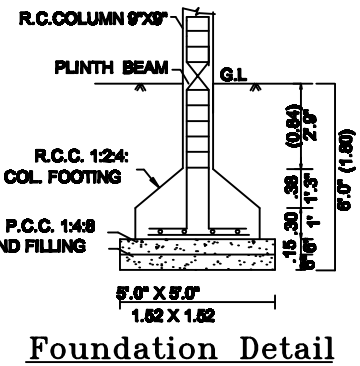
Foundation Detail
