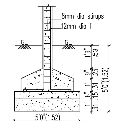
COLUMN FOUNDATION DETAIL
