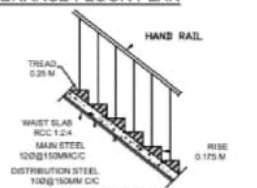
STAIR CASE DETAILS SCALE 1:300
