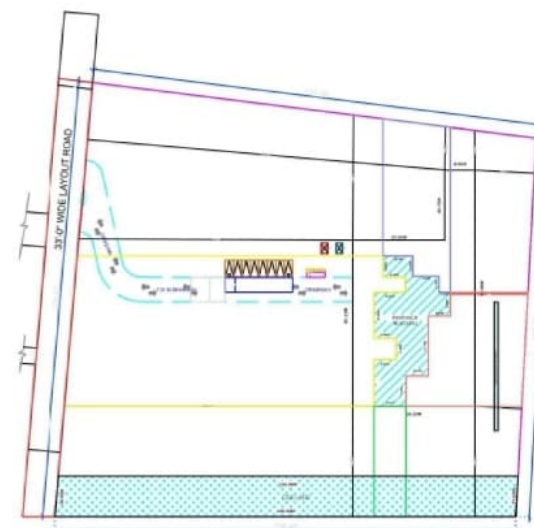
SITE PLAN [1:500]
