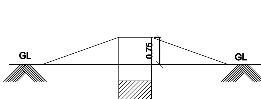
Dwarf Wall Details
