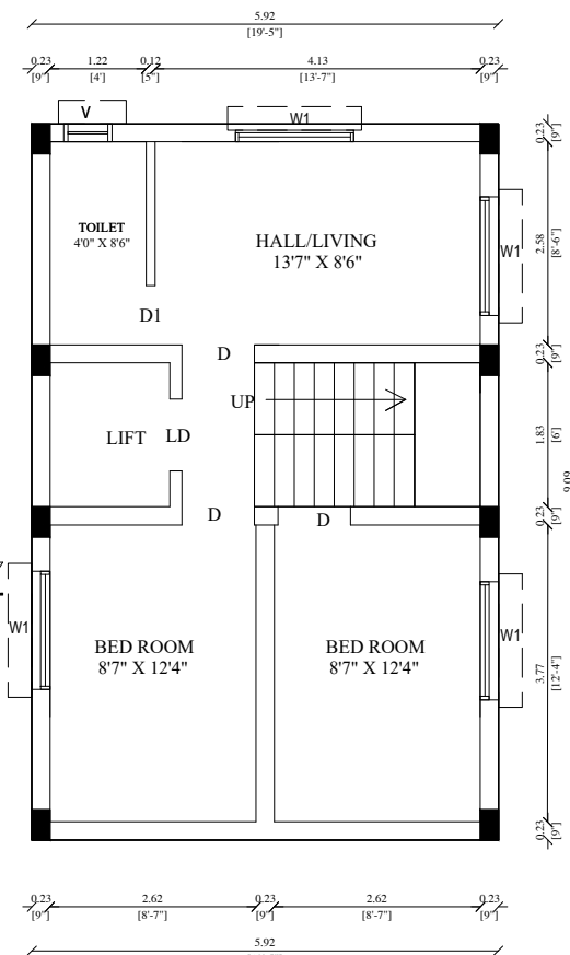
PRO.THIRD FLOOR PLAN
