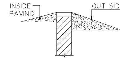
DWARF WALL SECTION
