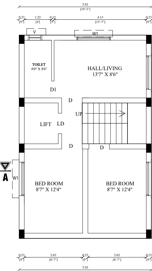
PRO.SECOND FLOOR PLAN
