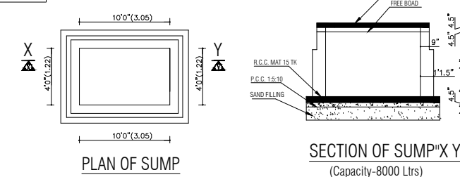
PLAN OF SUMP
