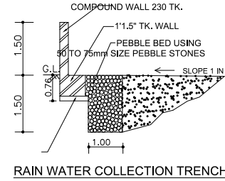
RAIN WATER COLLECTION TRENCH
