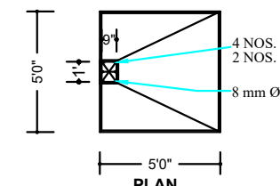
END WALL FOUNDATION
