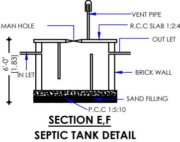
SECTION E,F SEPTIC TANK DETAIL
