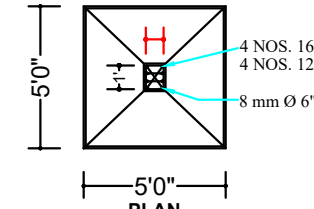
DETAIL OF COLUMN C1,C2
