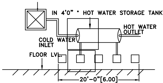
SOLAR HOT WATER SYSTEM DETAIL
