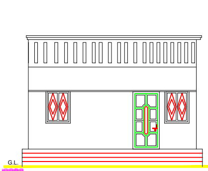
FRONT ELEVATION (PROPOSED)
