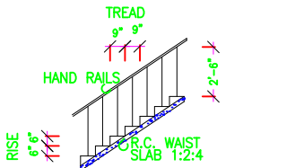
STAIRCASE DETAILS
