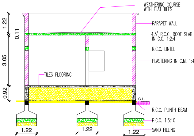
SECTION ON 'AA' (PROPOSED)
