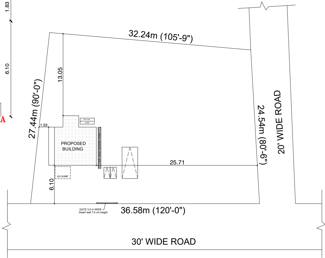
SITE & KEY PLAN SCALE:1:400
