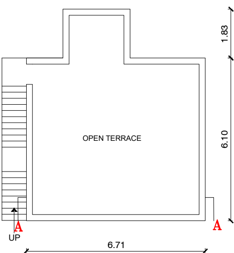
TERRACE FLOOR PLAN (PROPOSED)
