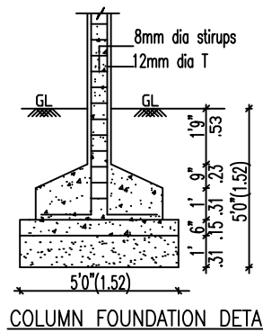
COLUMN FOUNDATION DETAIL SCALE 1"=4'0"(1:50)
