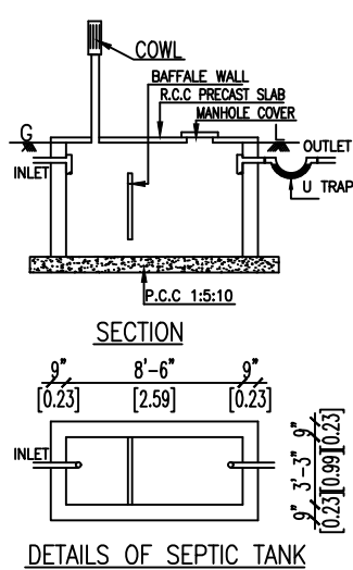
DETAILS OF SEPTIC TANK
