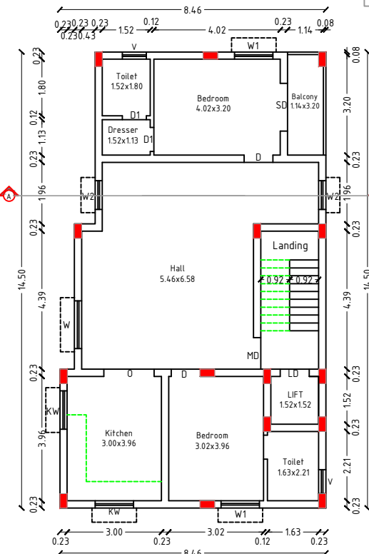
TYPICAL FLOOR PLAN FIRST, SECOND & THIRD
