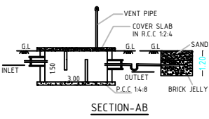
SECTION-AB
