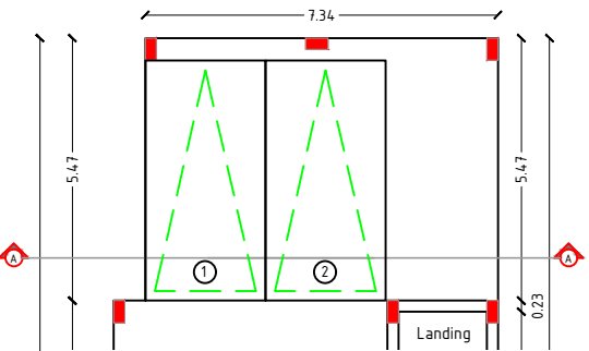
TYPICAL FLOOR PLAN FIRST, SECOND & THIRD
