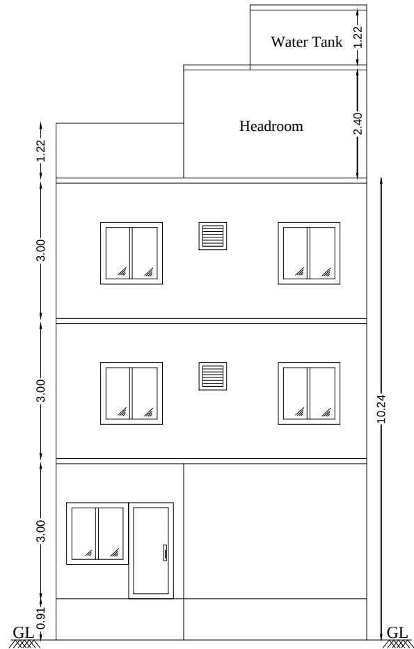
FRONT ELEVATION
