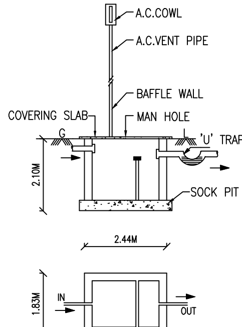
SEPTIC TANK
