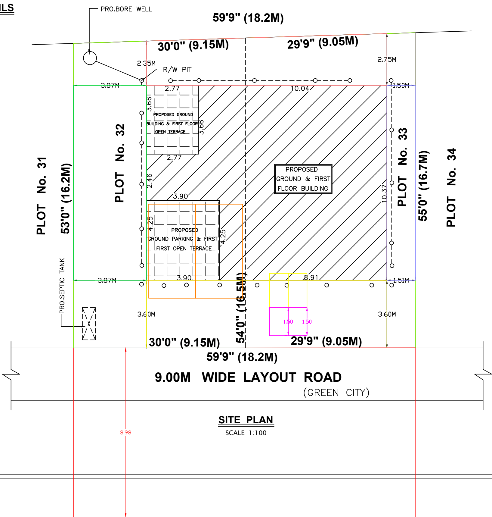
LAYOUT BOUNDRY
