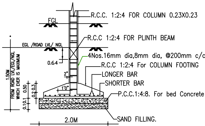
FOUNDATION DETAILS
