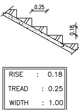
STAIRS DETAILS
