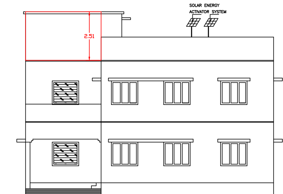
FRONT ELEVATION
