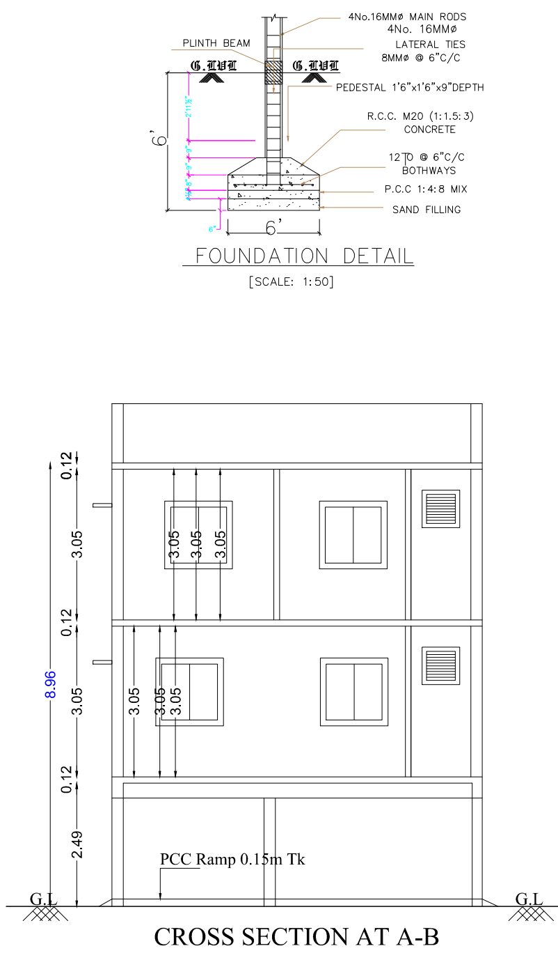
CROSS SECTION AT A-B
