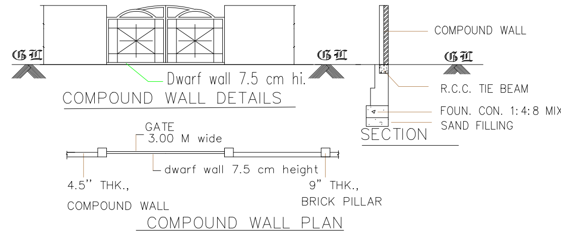
COMPOUND WALL PLAN
