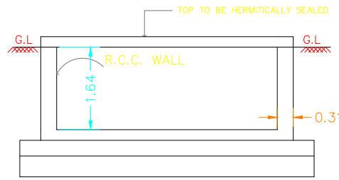
RWH SECTION RWH_CAPACITY_L = 2000LTRS
