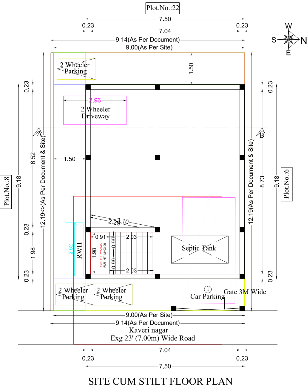
SITE CUM STILT FLOOR PLAN
