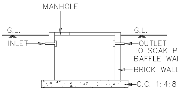
SECTION OF UG SUMP
