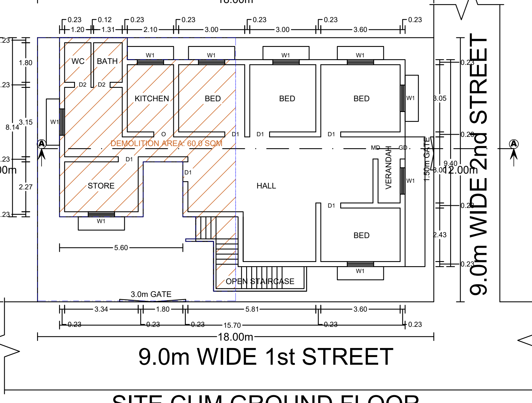
SITE CUM GROUND FLOOR (TO BE DEMOLISHED)
