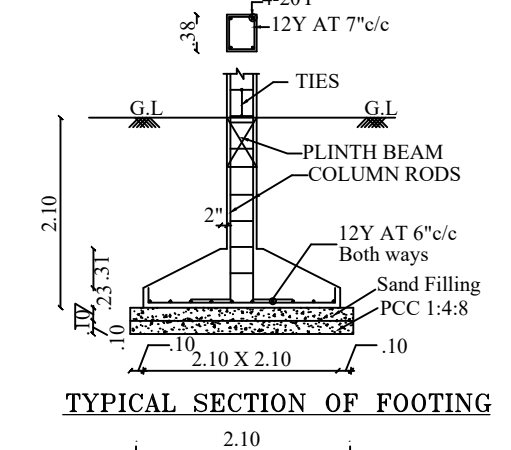
TYPICAL SECTION OF FOOTING
