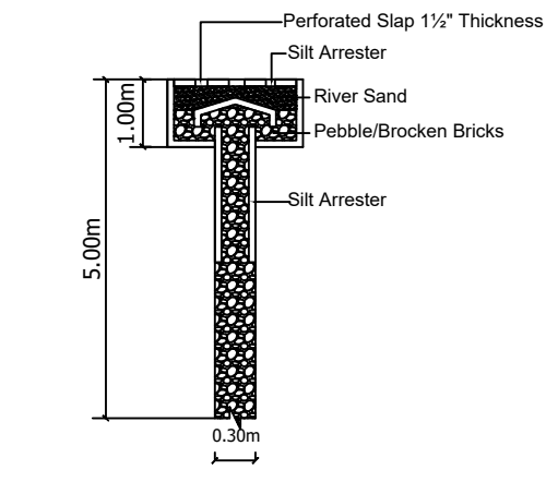
PERCOLATION PIT
