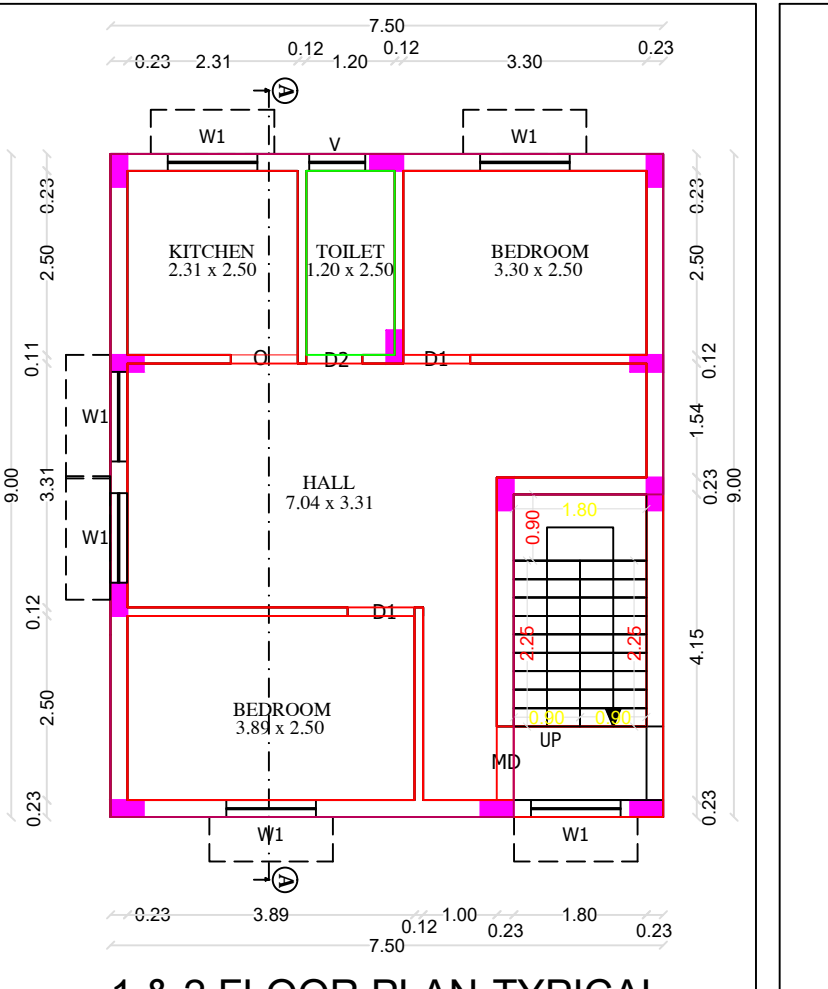
1 & 2 FLOOR PLAN-TYPICAL
