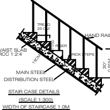
STAIR CASE DETAILS (SCALE 1:300)
