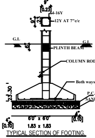
TYPICAL SECTION OF FOOTING
