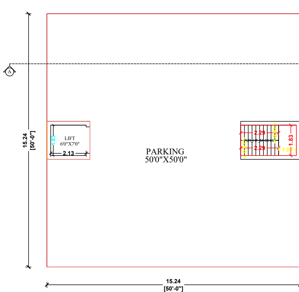
PROPOSED STILT FLOOR PLAN
