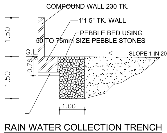
RAIN WATER COLLECTION TRENCH
