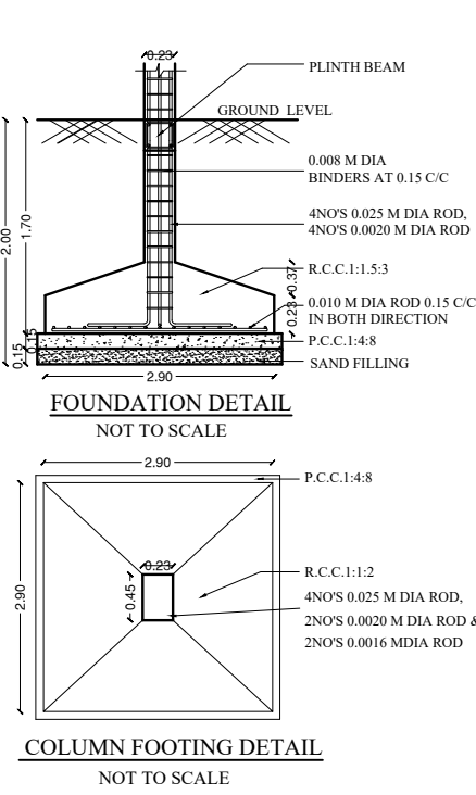
COLUMN FOOTING DETAIL NOT TO SCALE
