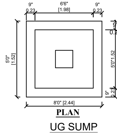
PLAN UG SUMP
