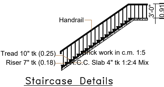
Staircase Details
