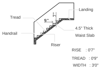
STAIRCASE DETAIL
