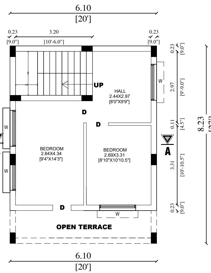
PRO.SECOND FLOOR
