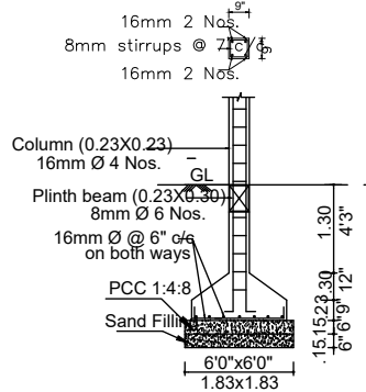
FOUNDATION DETAIL
