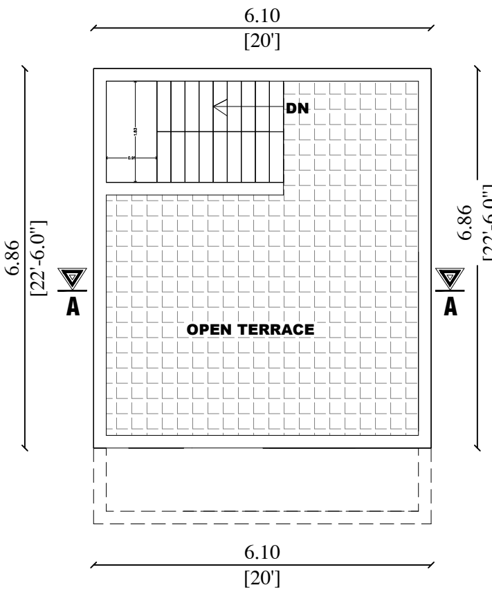
PRO.TERRACE FLOOR
