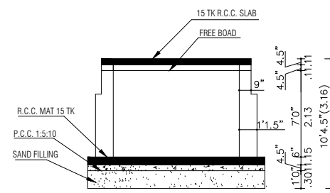
SECTION OF SUMP "X-Y" (Capacity-8000 Ltrs)
