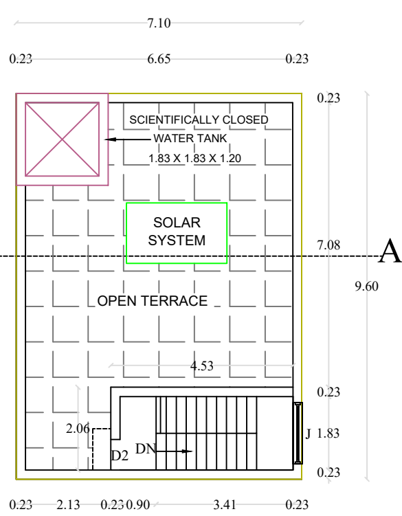
TERRACE FLOOR
