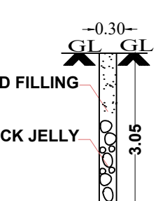
PERCOLATION PIT
