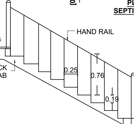
STAIRCASE DETAIL
