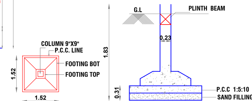
PLAN OF FOOTING
