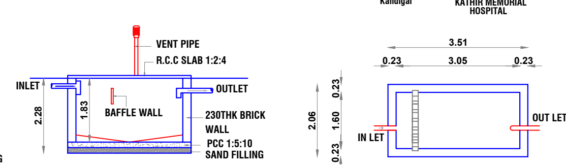
SECTION OF SEPTIC TANK
