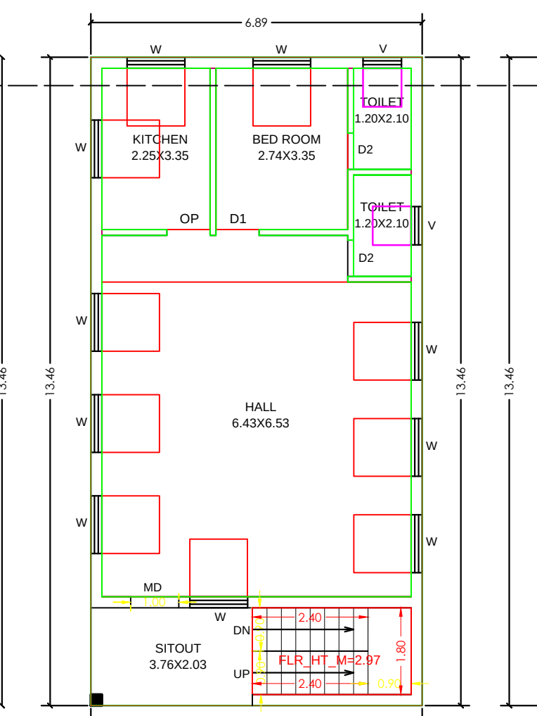
TYPICAL FLOOR PLAN=1,2 TYPICAL FLOOR PLAN=1,2
