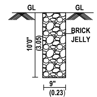
PERCOLATION PIT
