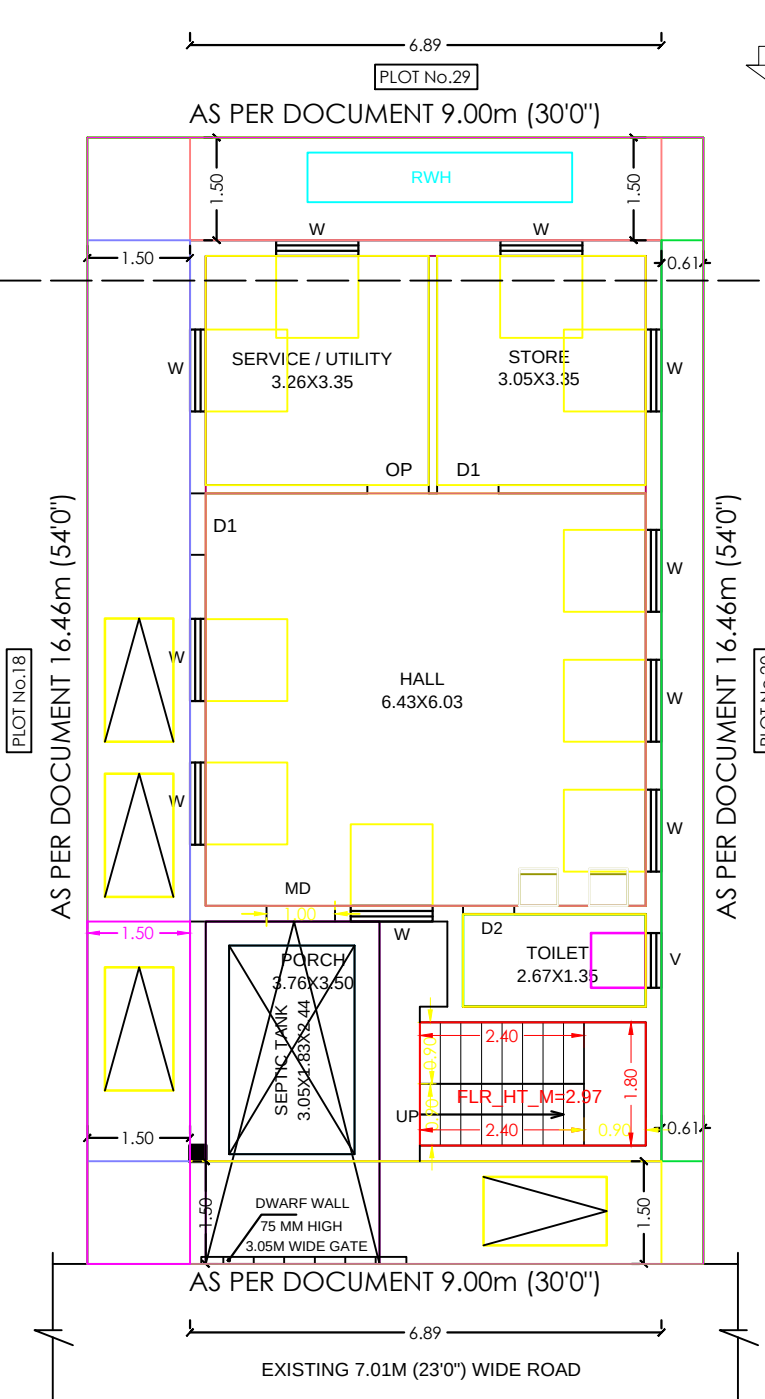
SITE / GROUND FLOOR PLAN.
