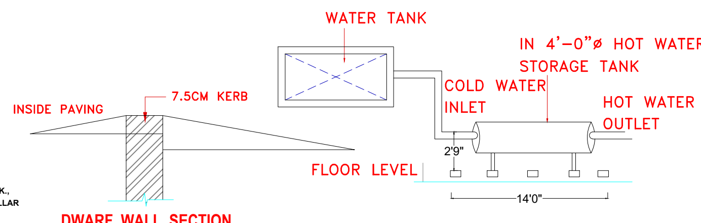
Solar Waterheater Detail
