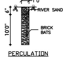
PERCOLATION PIT [N.T.S.]
