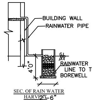
SEC. OF RAIN WATER HARVEST
