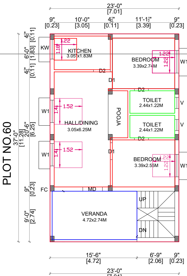
FIRST FLOOR PLAN (EXISTING BUILDING)
