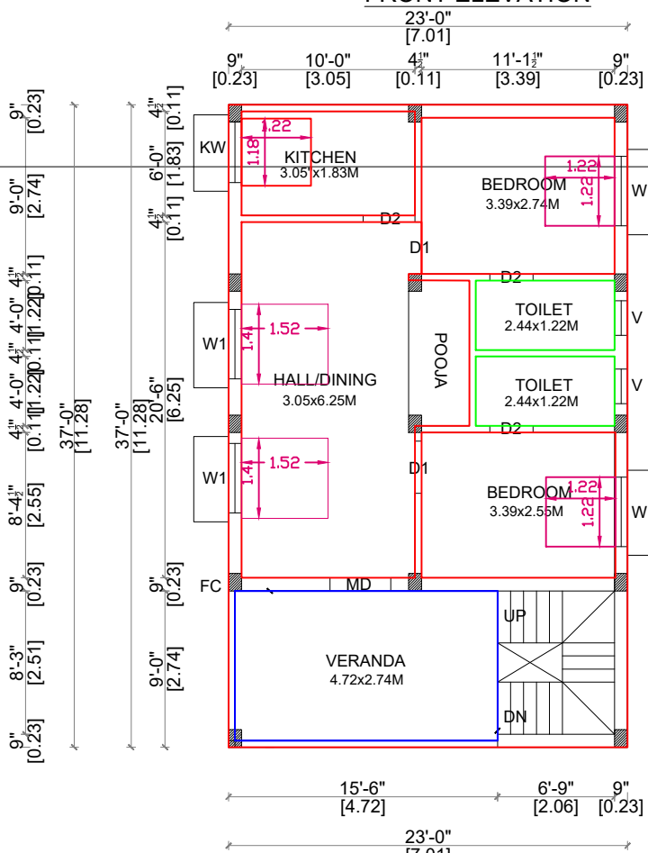
SECOND FLOOR PLAN (PROPOSED BUILDING)
