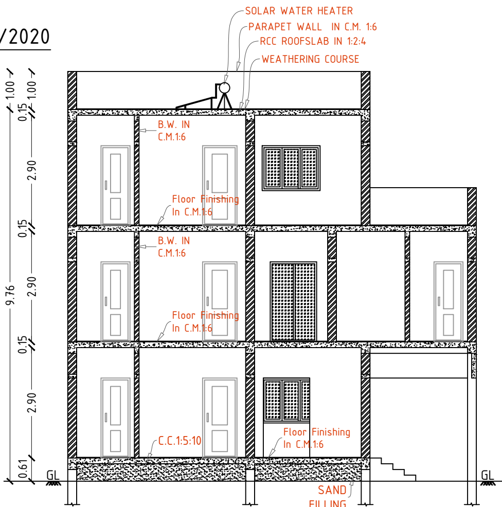
SECTION-A-A
