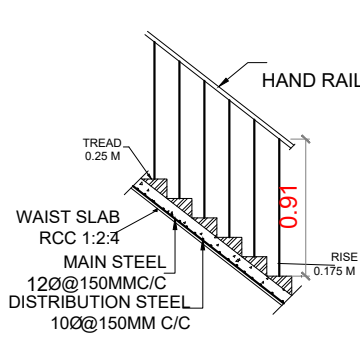
STAIR CASE DETAILS SCALE 1:300
