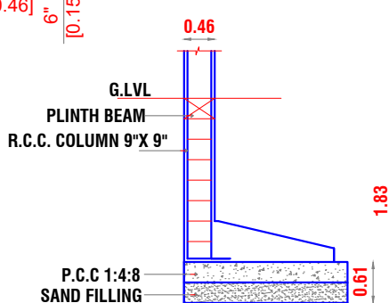
END FOOTING DETAILS
