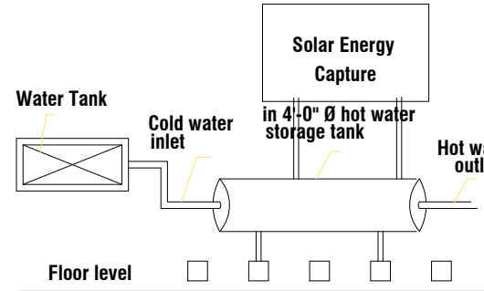
SOLAR HOT WATER SYSTEM
