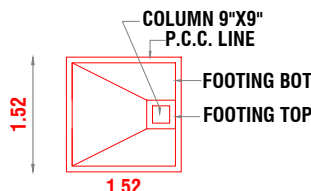
PLAN OF FOOTING
