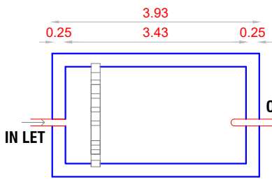
PLAN OF SEPTIC TANK CAPACITY - 8000 LITRES
