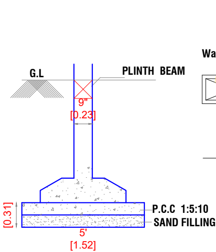
FOUNDATION DETAIL
