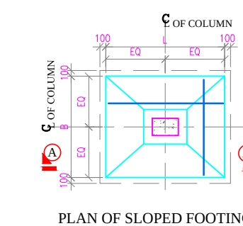
PLAN OF SLOPED FOOTING
