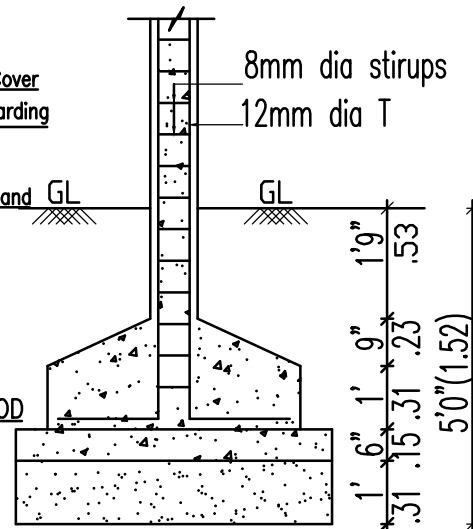
COLUMN FOUNDATION DETAIL
