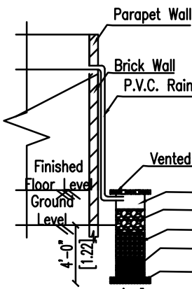
SECTION OF RAINWATER HARVESTING SYSTEM PERCOLATION TRENCH METHOD
