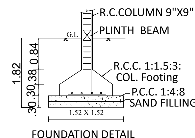
FOUNDATION DETAIL
