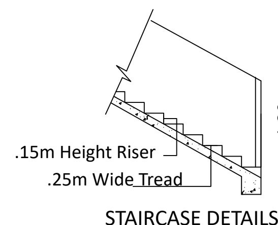
STAIRCASE DETAILS
