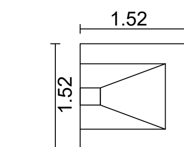
ECCENTRIC FOUNDATION PLAN
