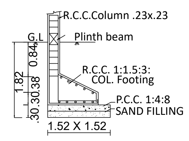
FOUNDATION DETAIL
