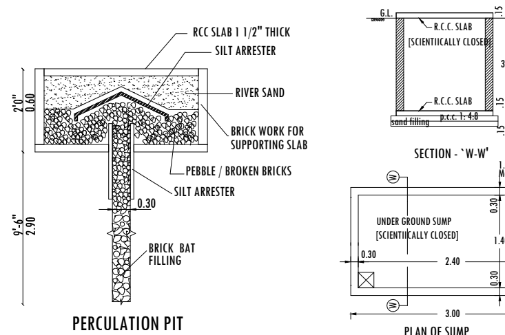
PERCOLATION PIT (Scale 1:50)
