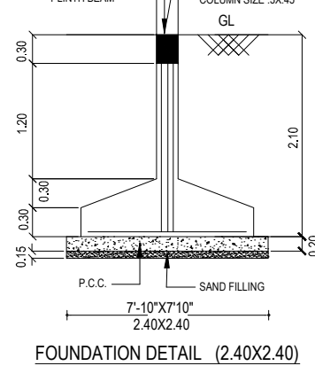
FOUNDATION DETAIL (2.40X2.40)
