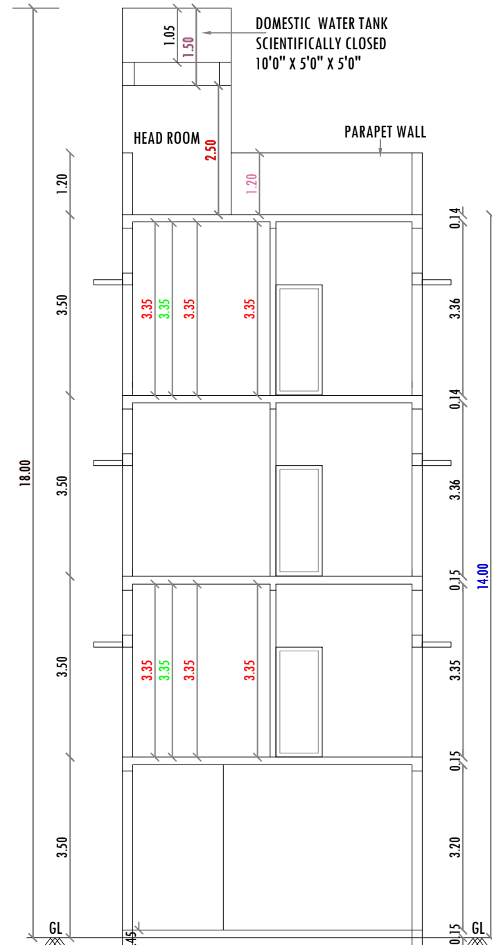
SECTION ON 'A-A' (PROPOSED)
