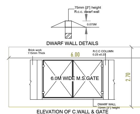
DWARF WALL DETAILS (Scale 1:50)
