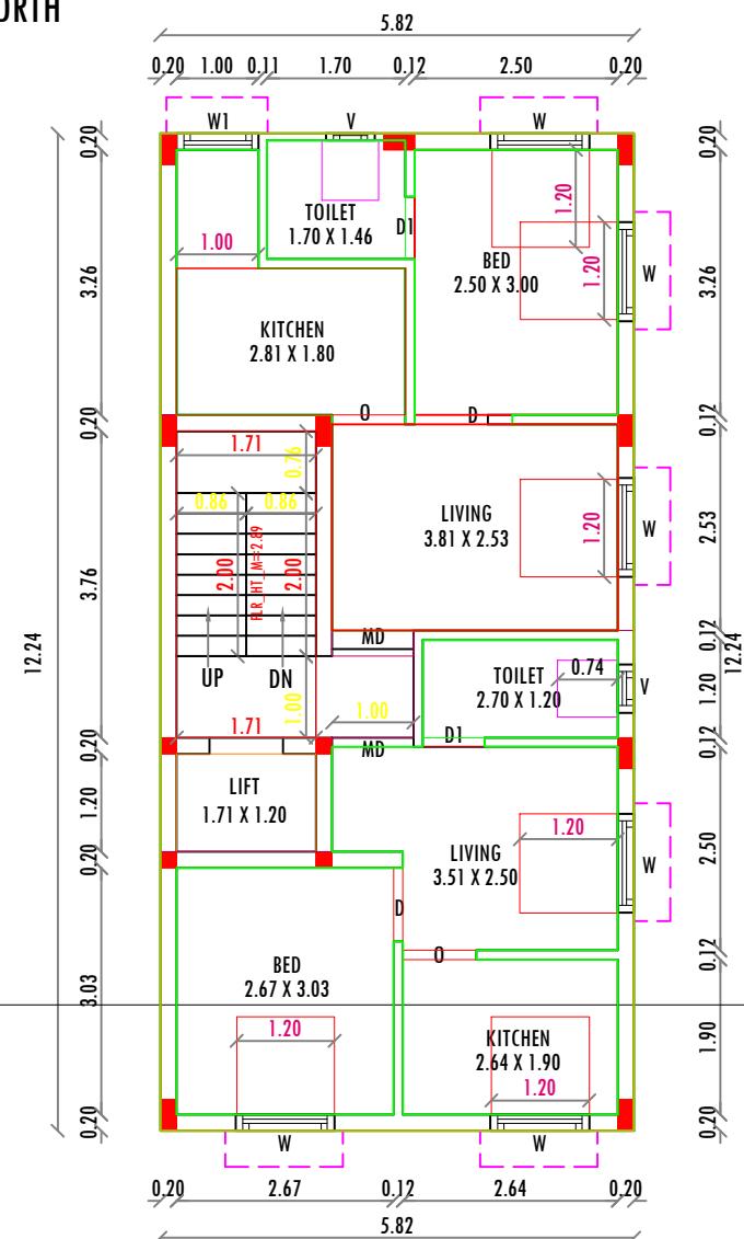
TYPICAL FIRST & SECOND FLOOR PLAN (PROPOSED)
