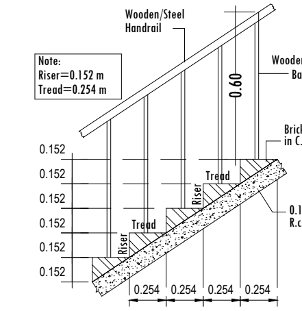
STAIRCASE DETAILS (Scale 1:25)
