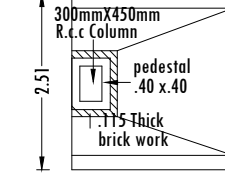
PLAN OF END WALL R.C.C. COLUMN FOUNDATION DETAILS (SCALE 1:50)
