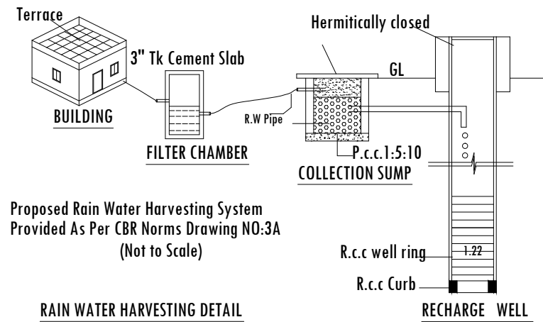
RAIN WATER HARVESTING DETAIL (Scale 1:25)
