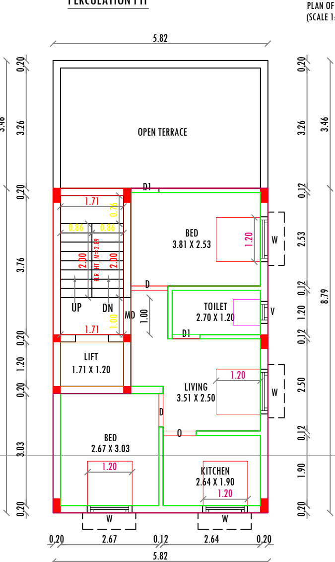
THIRD FLOOR PLAN (PART) (PROPOSED)
