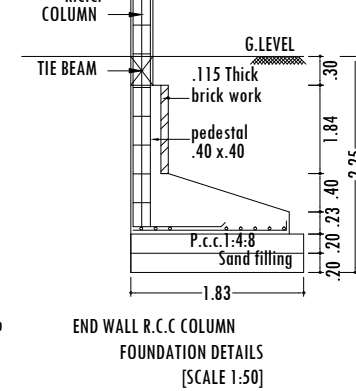
END WALL R.C.C. COLUMN FOUNDATION DETAILS (SCALE 1:50)
