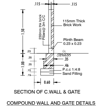
SECTION OF C.WALL & GATE COMPOUND WALL AND GATE DETAILS
