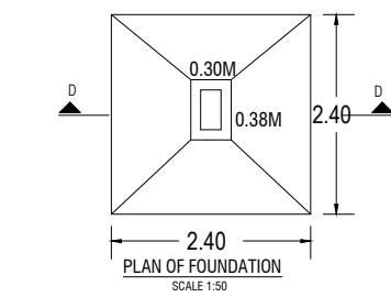
PLAN OF FOUNDATION (SCALE 1:50)
