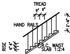
STAIRCASE DETAILS
