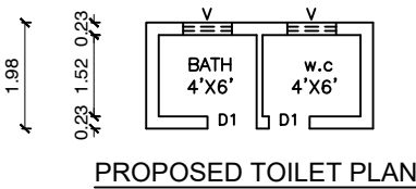
PROPOSED TOILET PLAN
