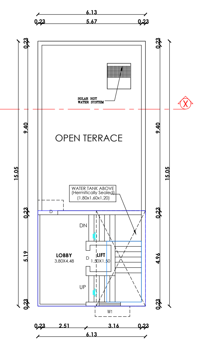
TERRACE FLOOR PLAN (PROPOSED)
