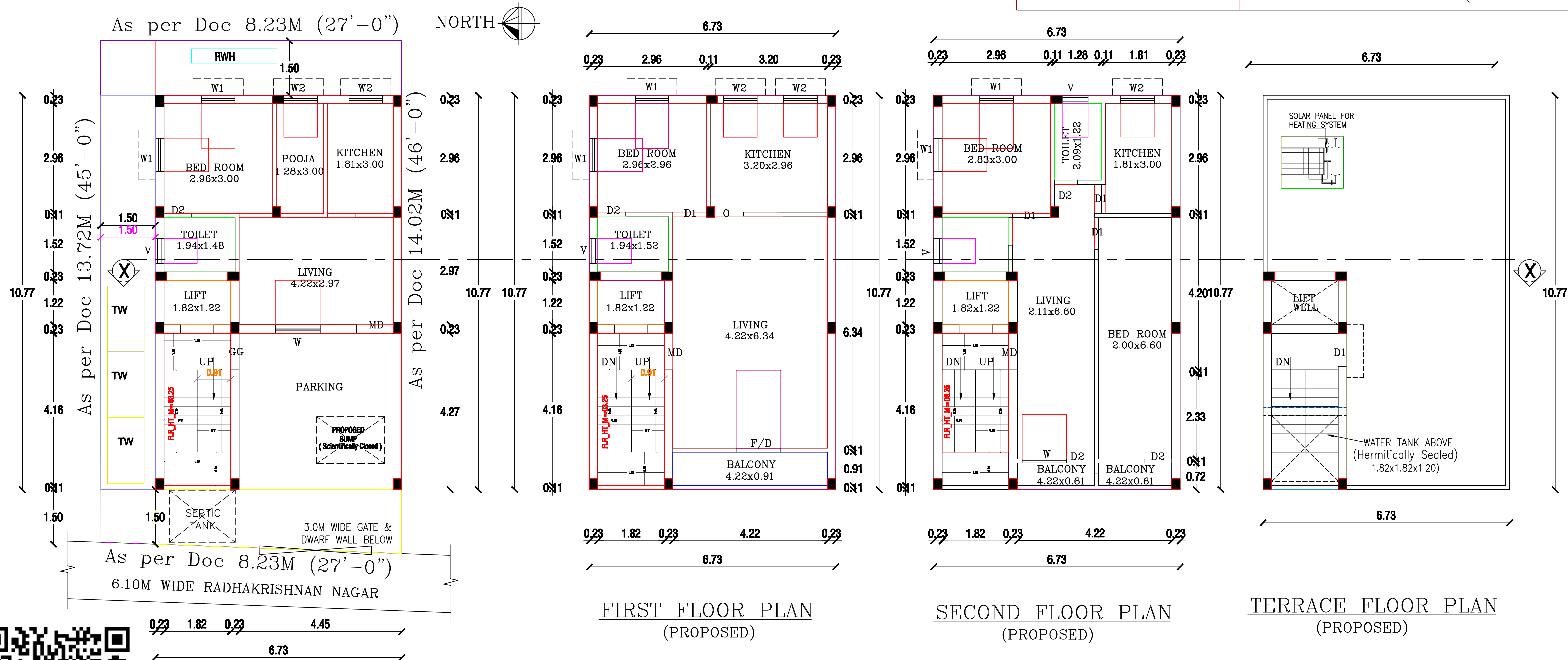
UM GROUND FLOOR PLAN (PROPOSED)
