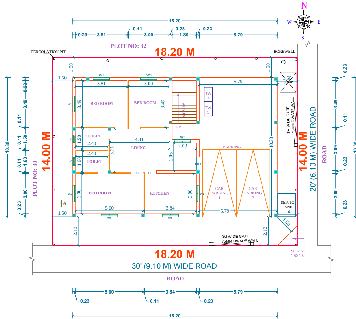
PROPOSED SITE CUM GROUND FLOOR PLAN
