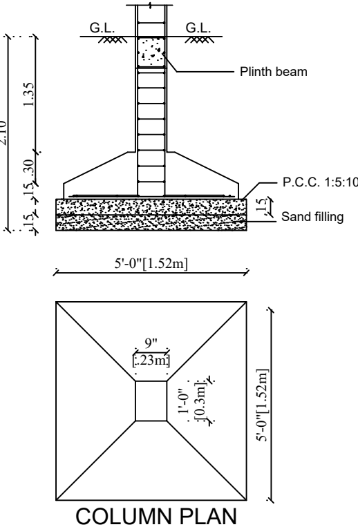
TYPICAL FOUNDATION DETAIL Footing Detail
