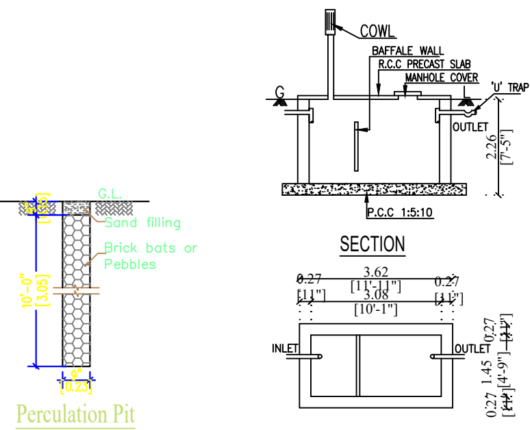
PLAN DETAILS OF SEPTIC TANK
