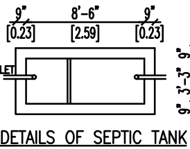
DETAILS OF SEPTIC TANK
