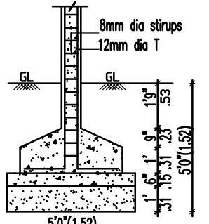
COLUMN FOUNDATION DETAIL
