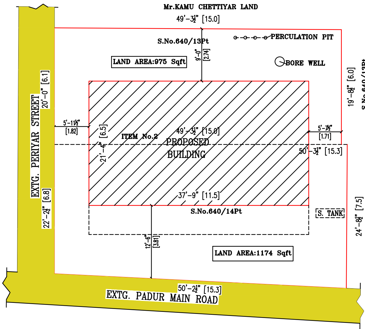
SITE PLAN
