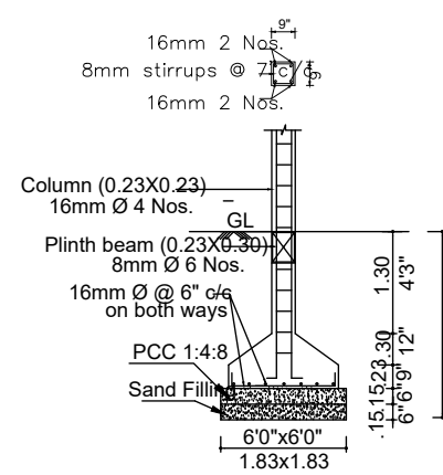
FOUNDATION DETAIL
