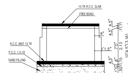
SECTION OF SUMP"X Y" (Capacity-8000 Ltrs)
