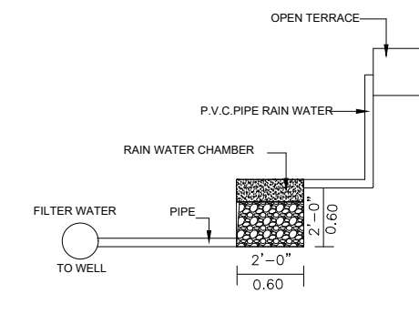
RAIN WATER HARVESTING
