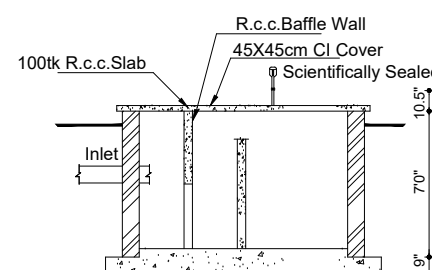
SECTION OF SEPTIC TANK "X Y"
