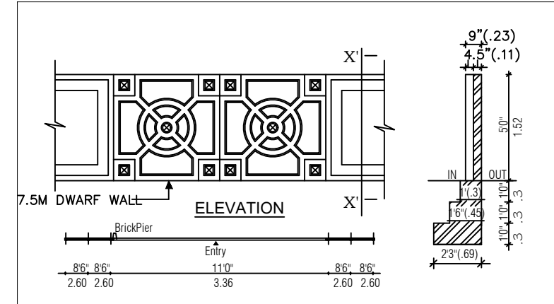
COMPOUND WALL IN PLAN SECTION ON "X-X"
