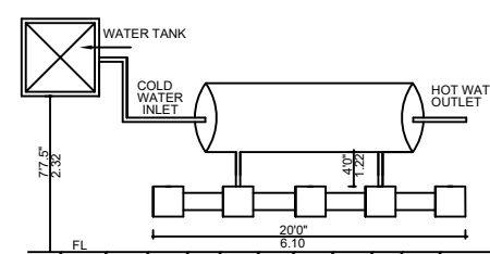
SOLOR HOT WATER SYSTEM DETAILS
