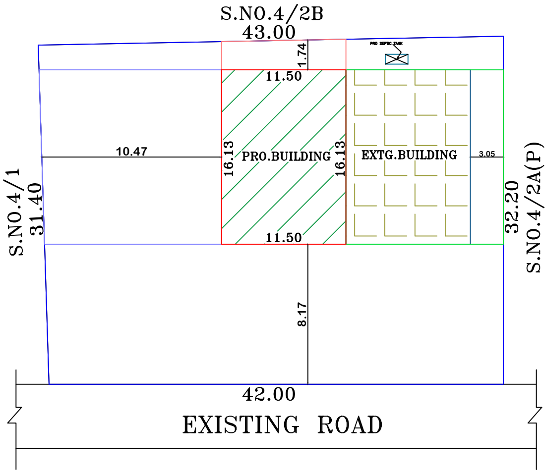
SITE PLAN
