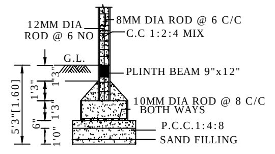
RUN THROUGH COLUMN FOUNDATION SCALE 1"=4'0" (1:50)
