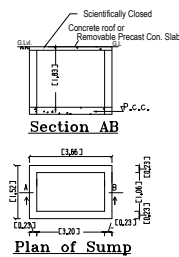
Plan of Sump
