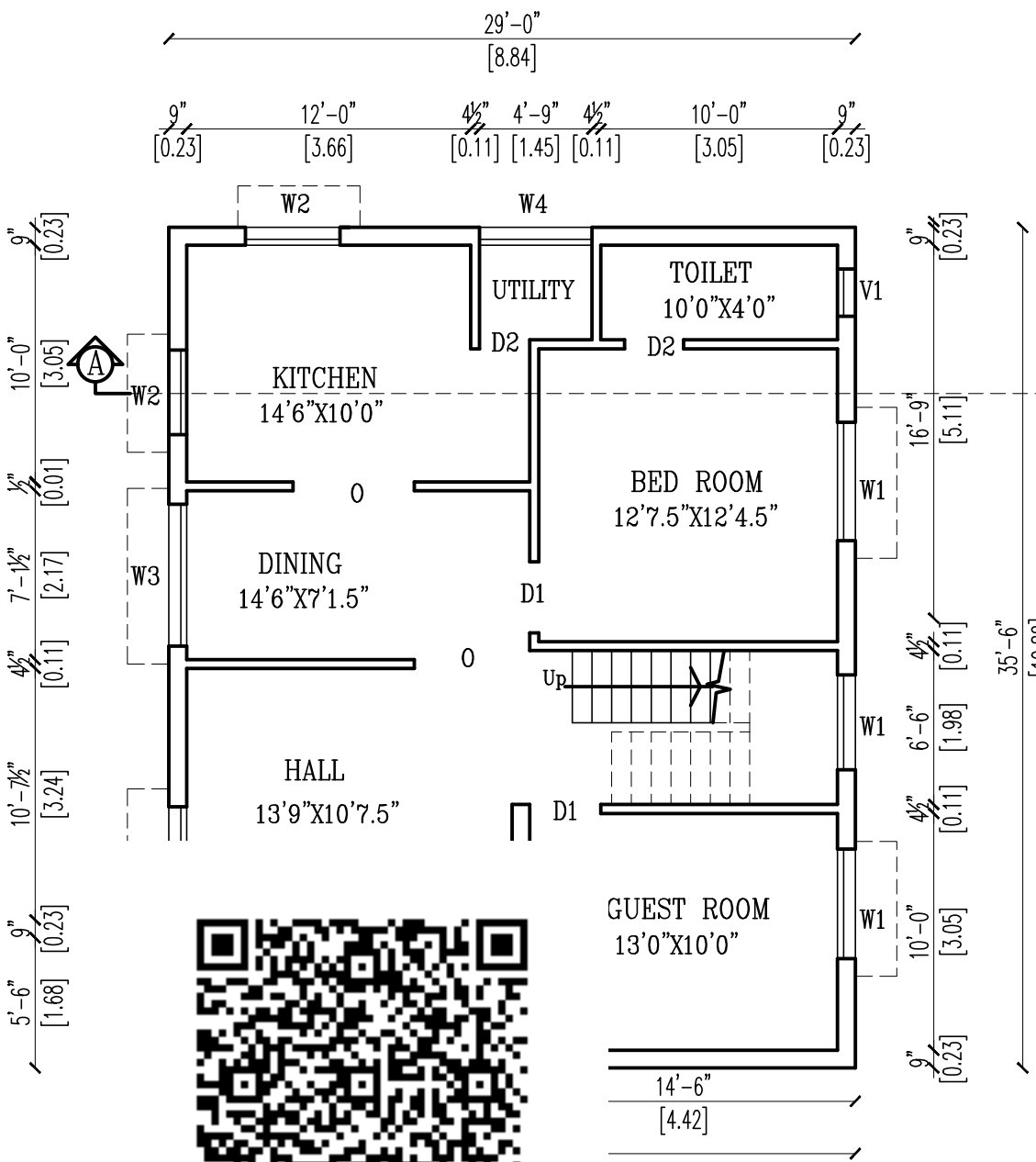
PRO. FLOOR PLAN
