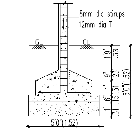
COLUMN FOUNDATION DETAIL
