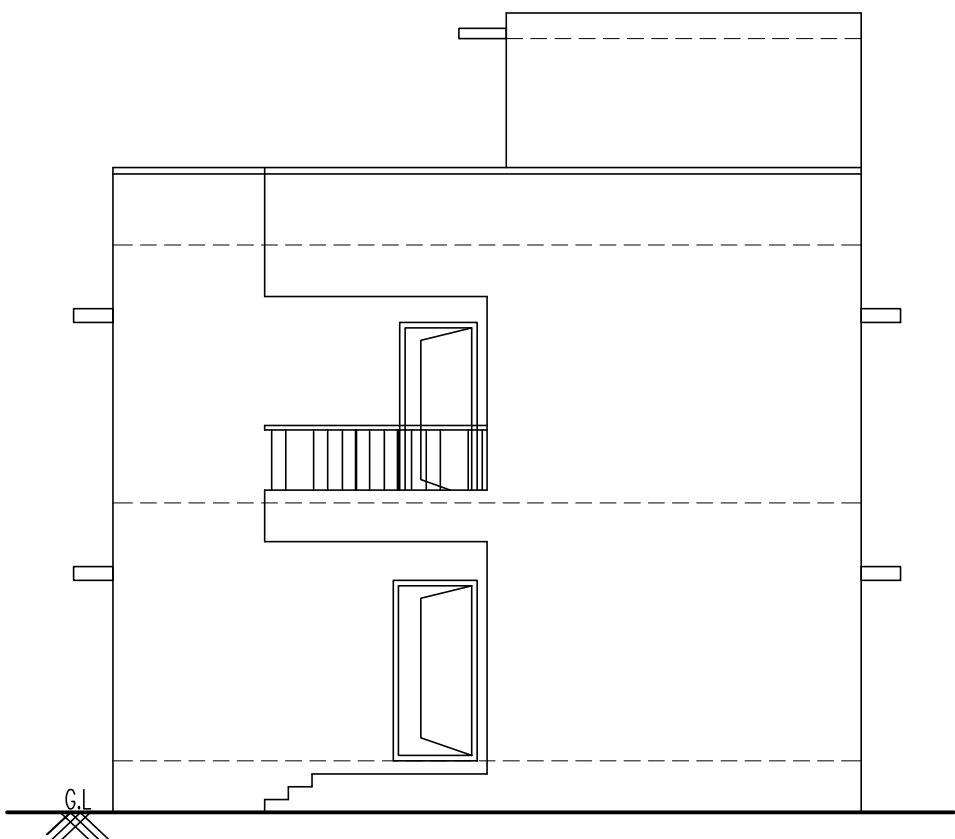
FRONT ELEVATION
