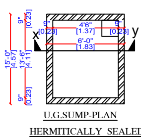
U.G. SUMP PLAN HERMITICALLY SEALED
