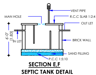
SECTION E.F. SEPTIC TANK DETAIL
