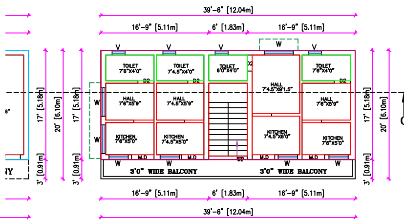
EXTG.FIRST FLOOR PLAN
