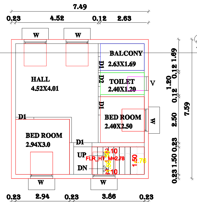
SCOND FLOOR PLAN PROPOSED
