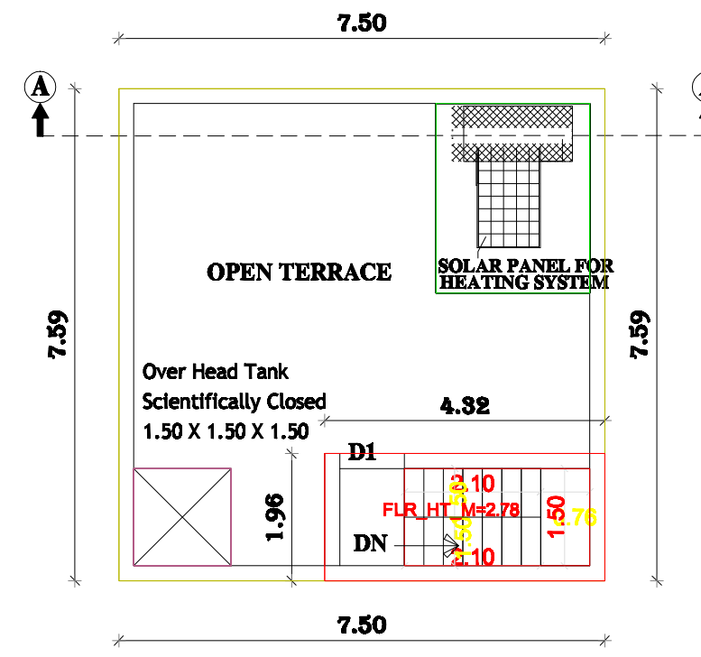
TERRACE FLOOR PLAN PROPOSED
